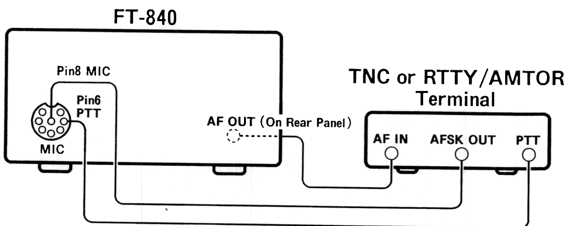
Packet TNC & RTTY/AMTOR Terminal Unit Interconnections
