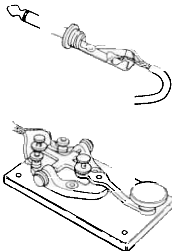
CW Key Connections
