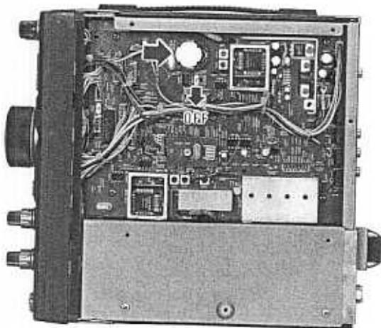
Fig. 6 Backup Switch
