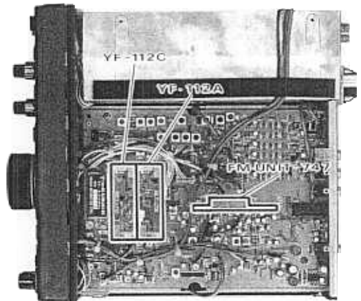
Figure 2: Filter & FM Unit Location
