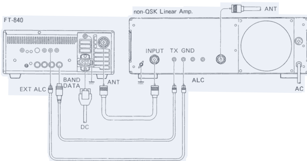
Other non-QSK Linear Amplifier
