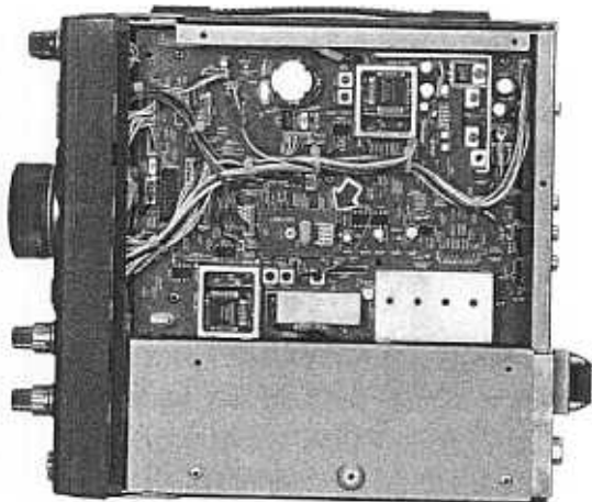
Fig. 4: TCXO-4 Installation
