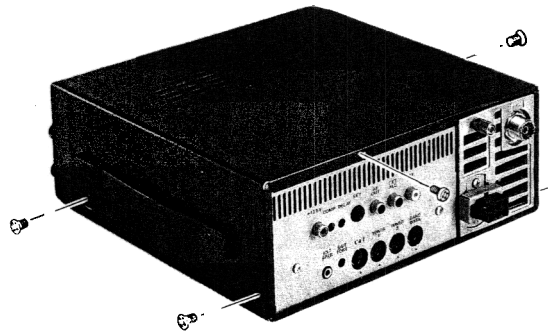
Figure 1: Top Cover Removal
