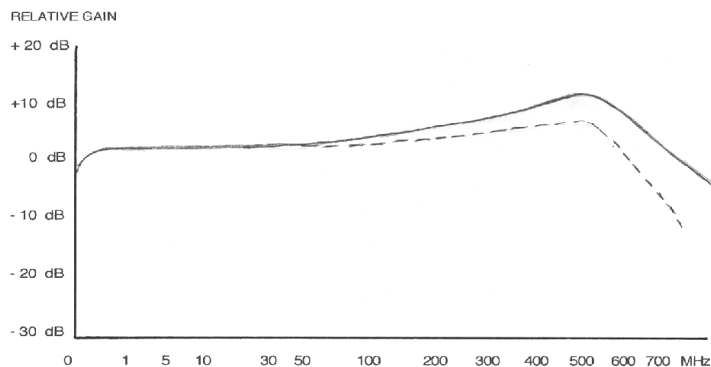
AMPLITUDE/FREQUENCY CHARACTERISTIC DX 500 ANTENNA
